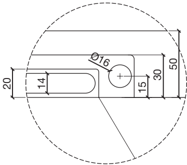
DETAIL F
