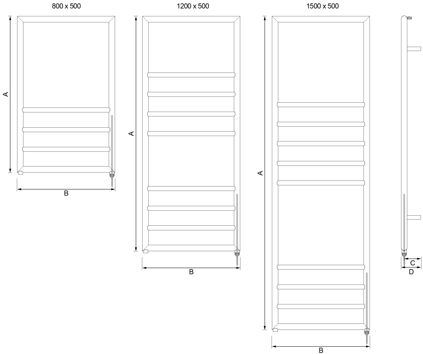
Front view
