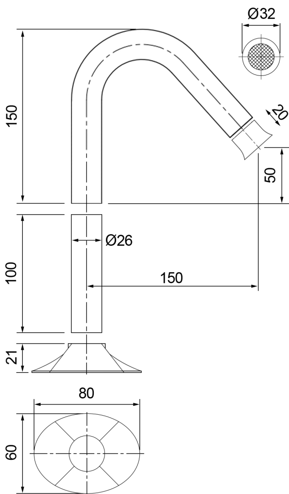
Bath filler spout
