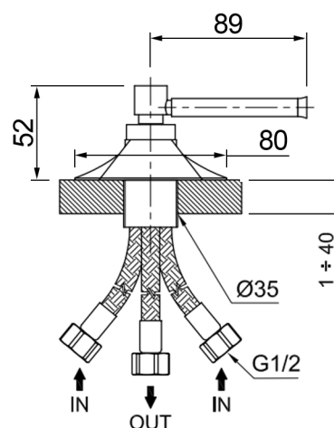
Mixer valve (handheld shower)
