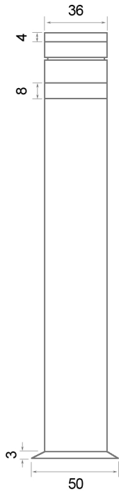
Front view
