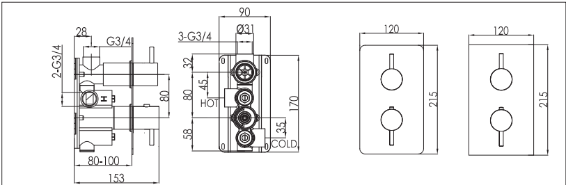
one-outlet
